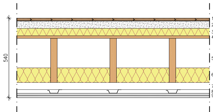
Figure 2.9. LVL joist floor structures for ground floors, intermediate floors and compartment floors.
