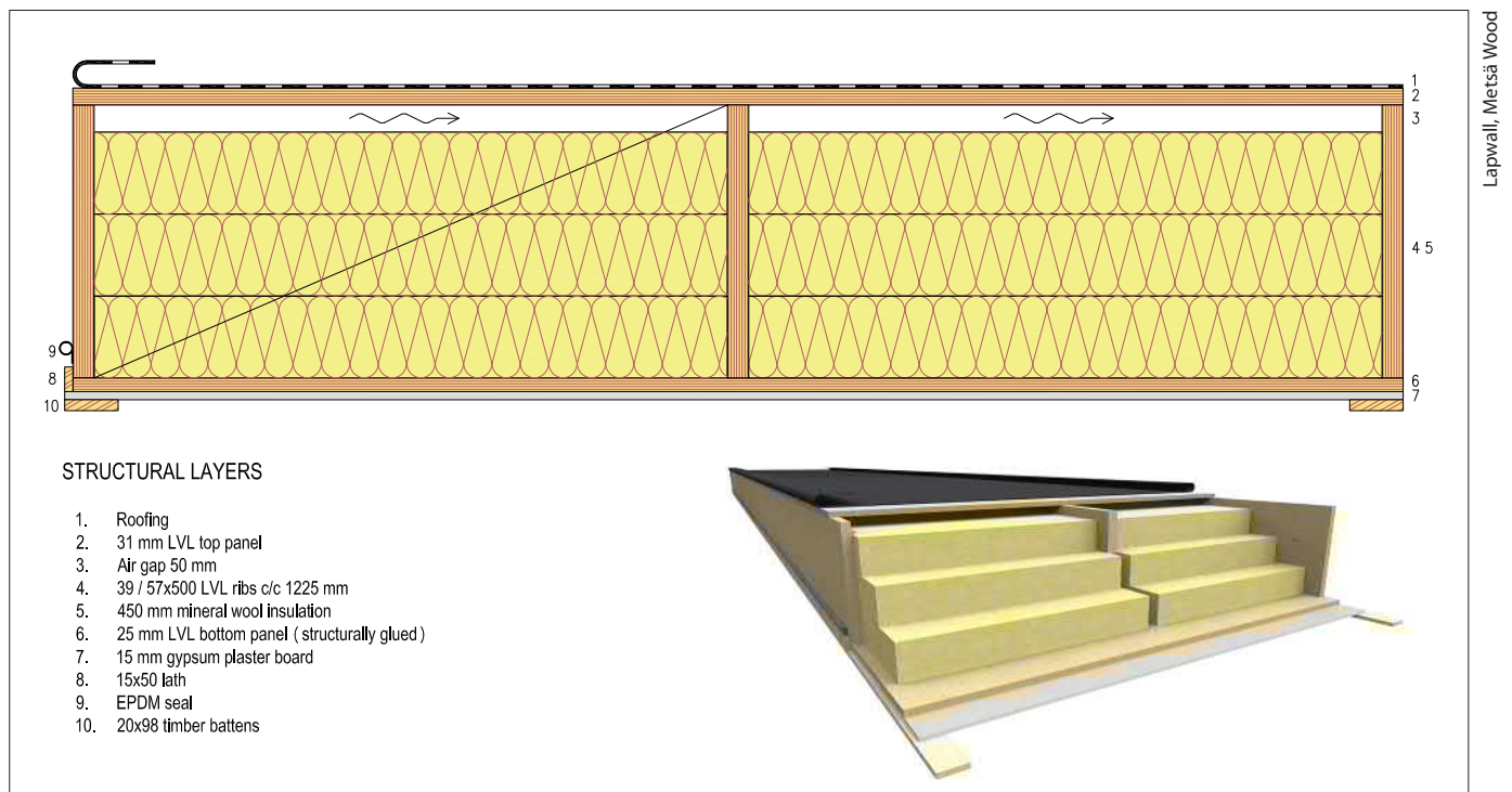
Figure 2.41. LVL box panel element.
