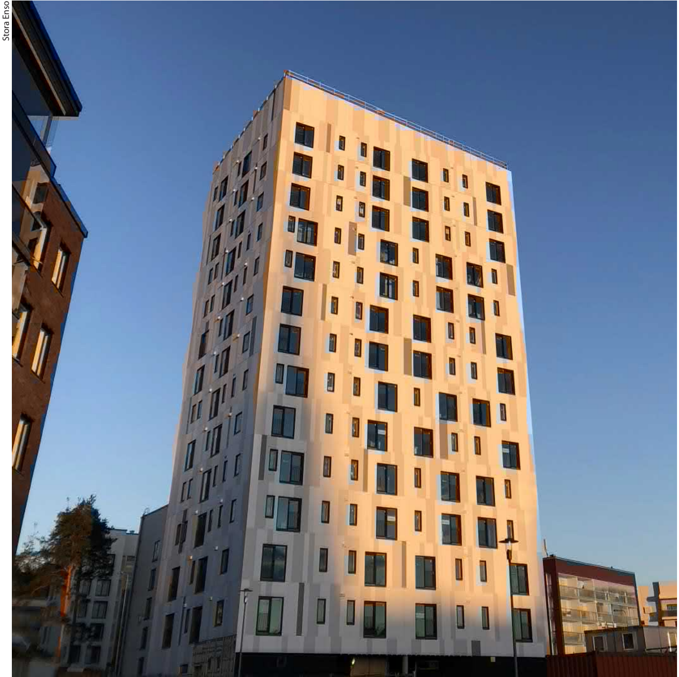
Figure 9.1. Wooden multi-storey building Lighthouse, Joensuu, Finland
