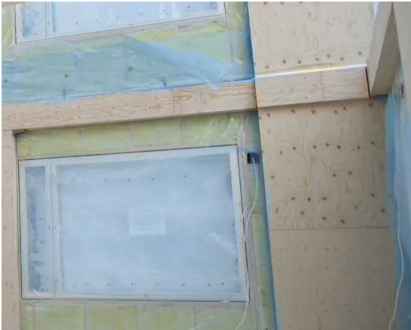
Figure 2.72. LVL-C bracing panels.
