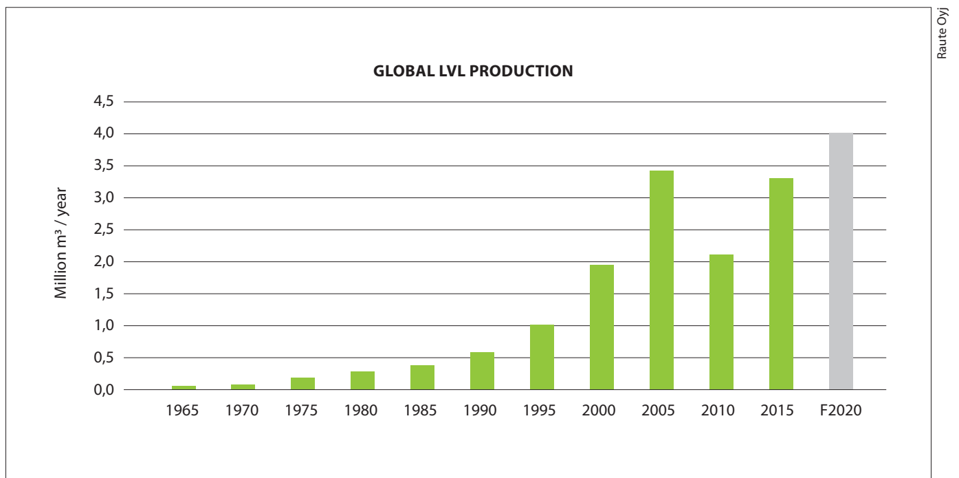
Figure 1.14 Development of structural LVL production volume globally 1965 – 2020 5 .
